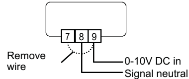
Figure 7: Wiring of external control signal
