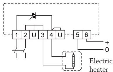
Supply voltage and load
